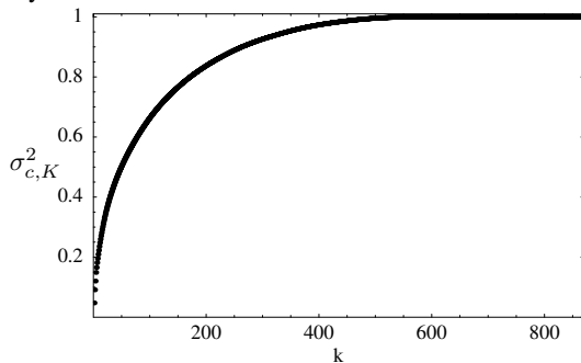
Figure 7: Eigenspectrum of the SUMO ontology sorted by value
